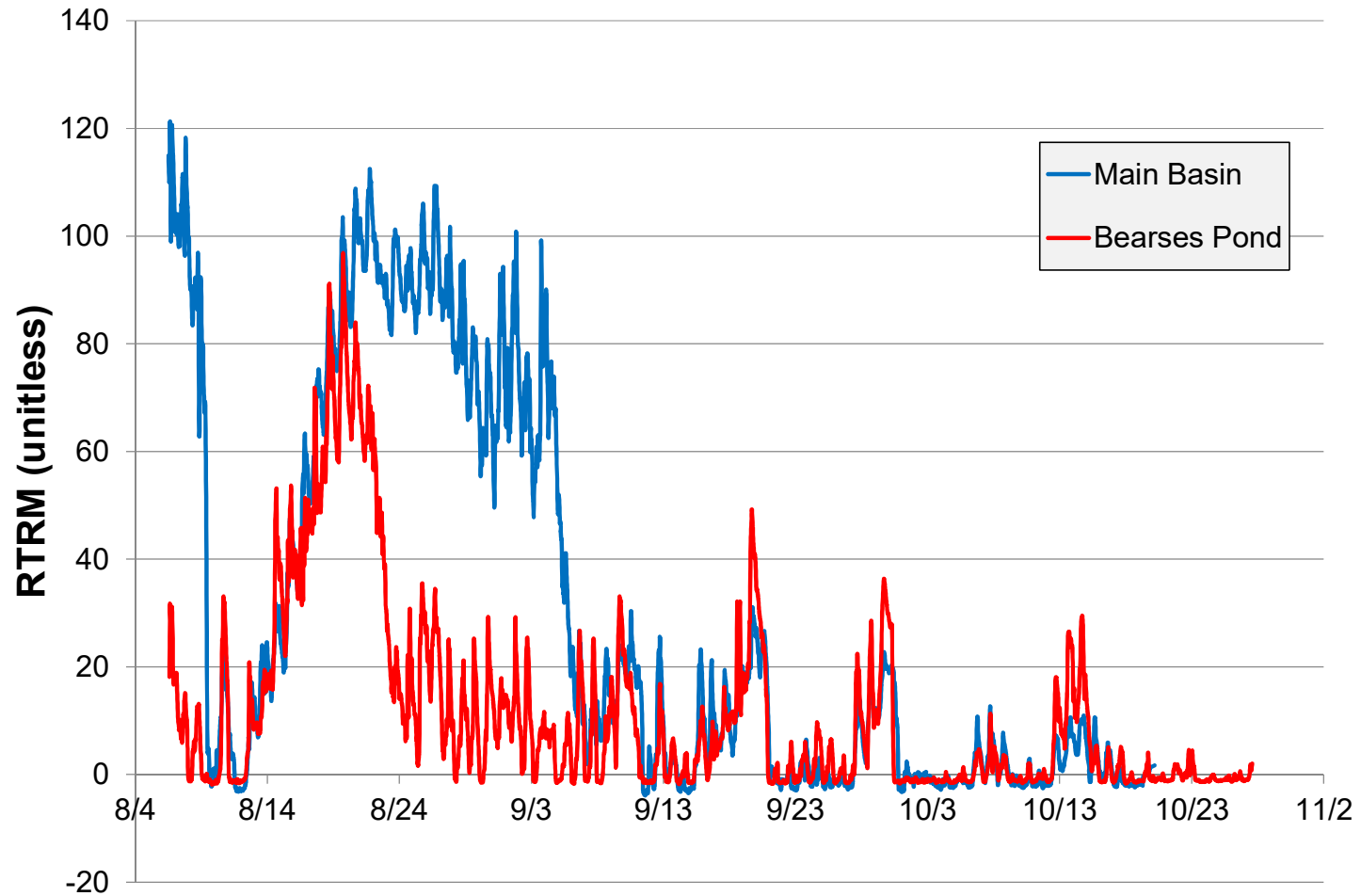
Figure 3. 2015 Relative Resistance to Thermal Mixing in Lake Wequaquet: Main Basin and Bearses Pond. Main Basin generally had high RTRM until early September, while Bearses Pond generally had low RTRM with brief periods (1-2 days) exceeding the RTRM threshold of 30 generally associated with temperature stratification and a more significant ~8 day period in mid-August.
