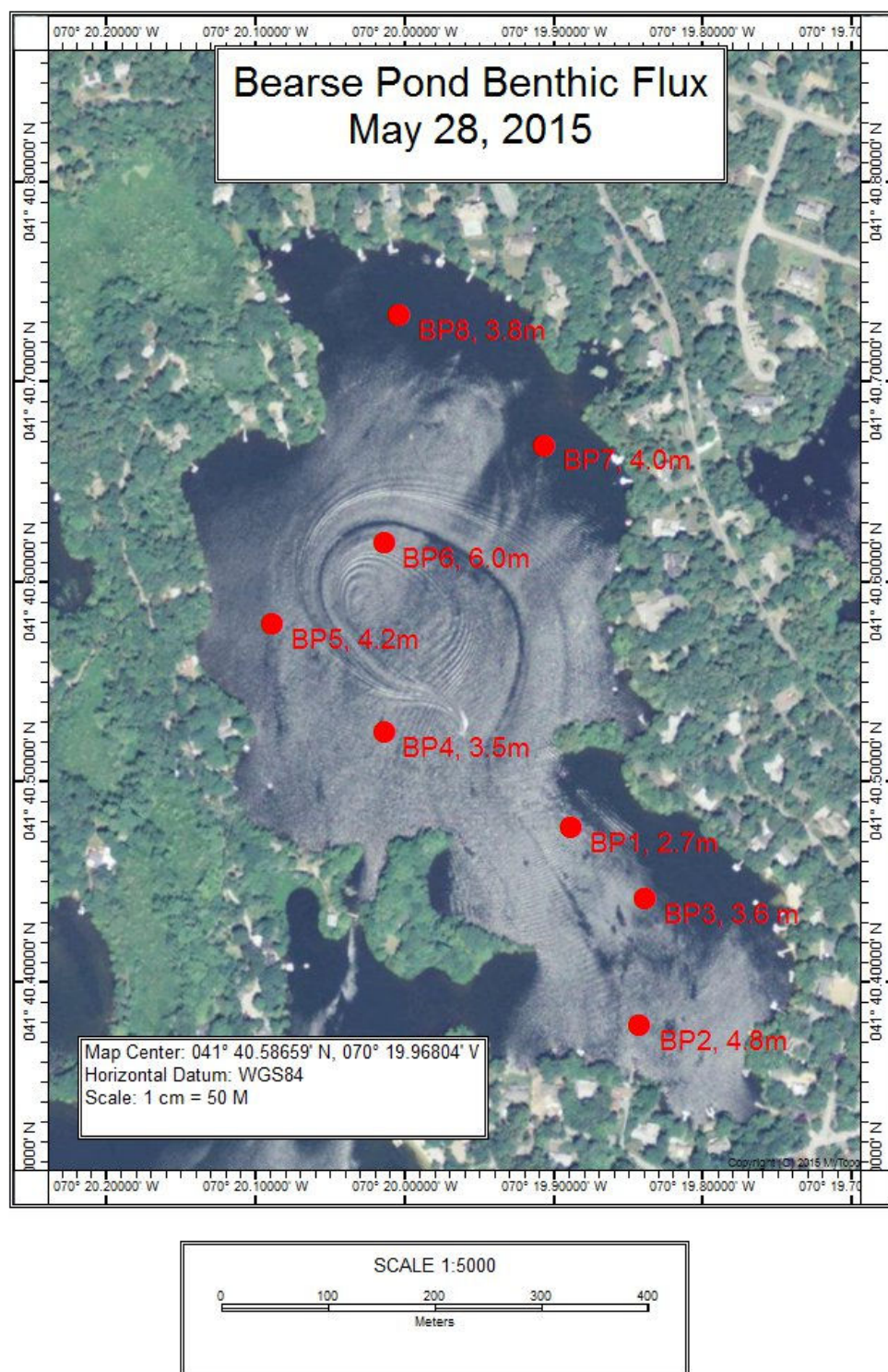
Figure 7. Sediment Core Collection Sites in Beares Pond. CSP-SMAST staff collected intact undisturbed cores from 8 locations on May 28, 2015. Cores were collected by SCUBA diver and were incubated at in situ temperatures to evaluate nutrient regeneration from the sediments under oxic and anoxic conditions using standard CSP-SMAST procedures.
