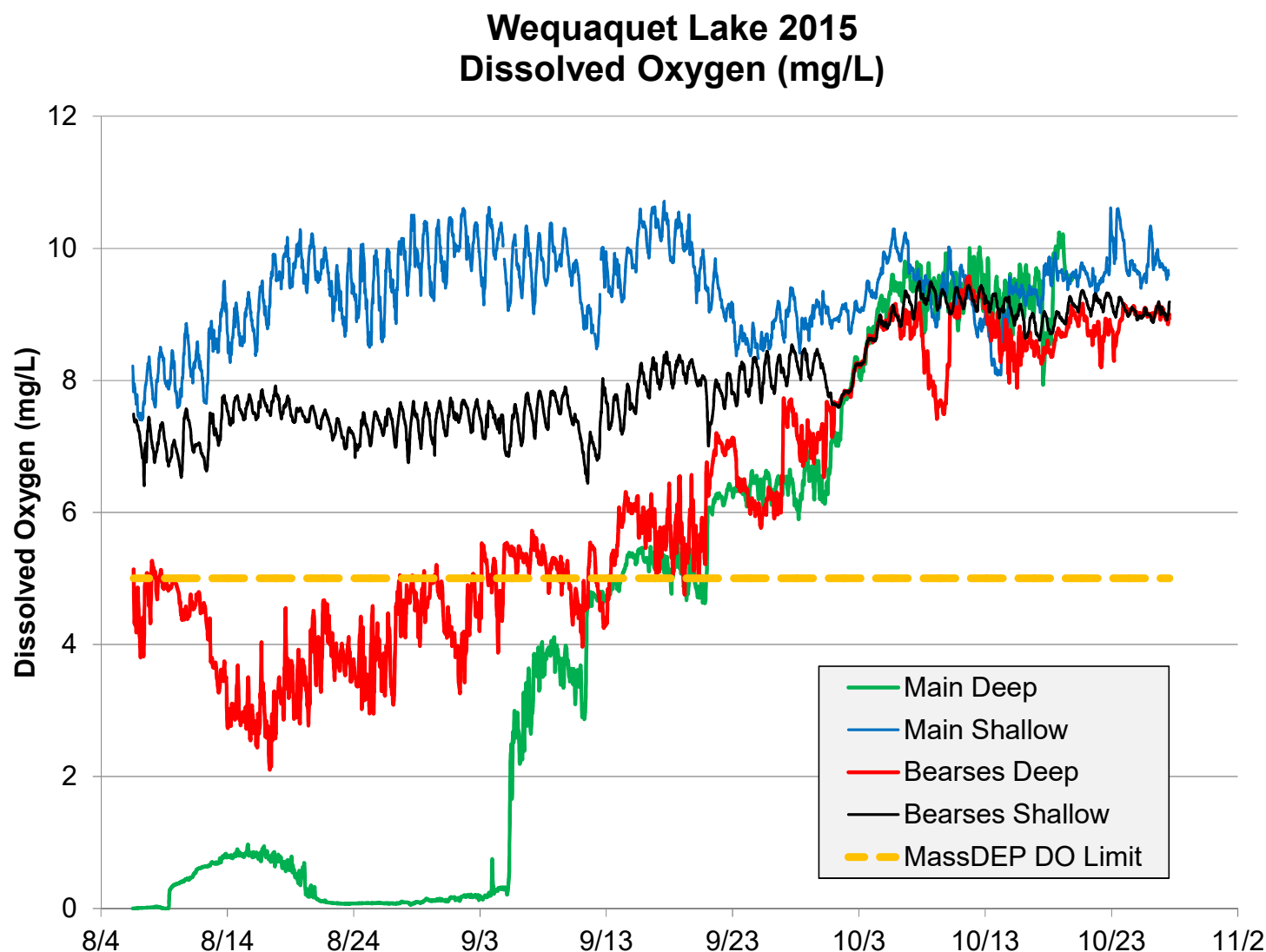
Figure 4. Lake Wequaquet 2015 Dissolved Oxygen Readings: Continuous Records in Main Basin and Bearses Pond. Recordings were collected between August 6 and October 27. Deep recordings in both basins (Bearses 4.6 m; Main 7.9 m) were generally below the MassDEP regulatory minimum of 5 mg/L until early September. Readings in the Main Basin were also generally anoxic and sufficiently prolonged to produce chemical phosphorus release from associated bottom sediments.
