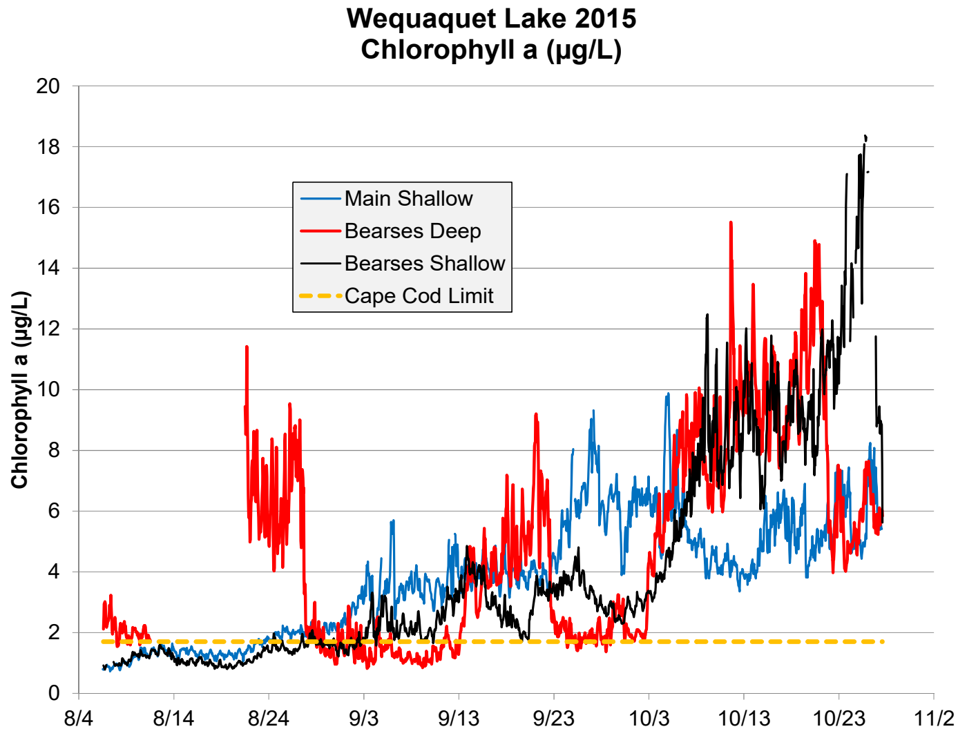
Figure 6. Lake Wequaquet 2015 Water-column Chlorophyll Readings: Continuous Records in Main Basin and Bearses Pond. Recordings were collected between August 6 and October 27, 2015. Shallow readings in both basins were notably low in August before rising above the Cape Cod ecoregion standard in September and nearly doubling again in October. Readings suggest that rooted plants were outcompeting phytoplankton in August and then reversed in September. Water-column was vertically well mixed in both basins from the last week in September to November.
