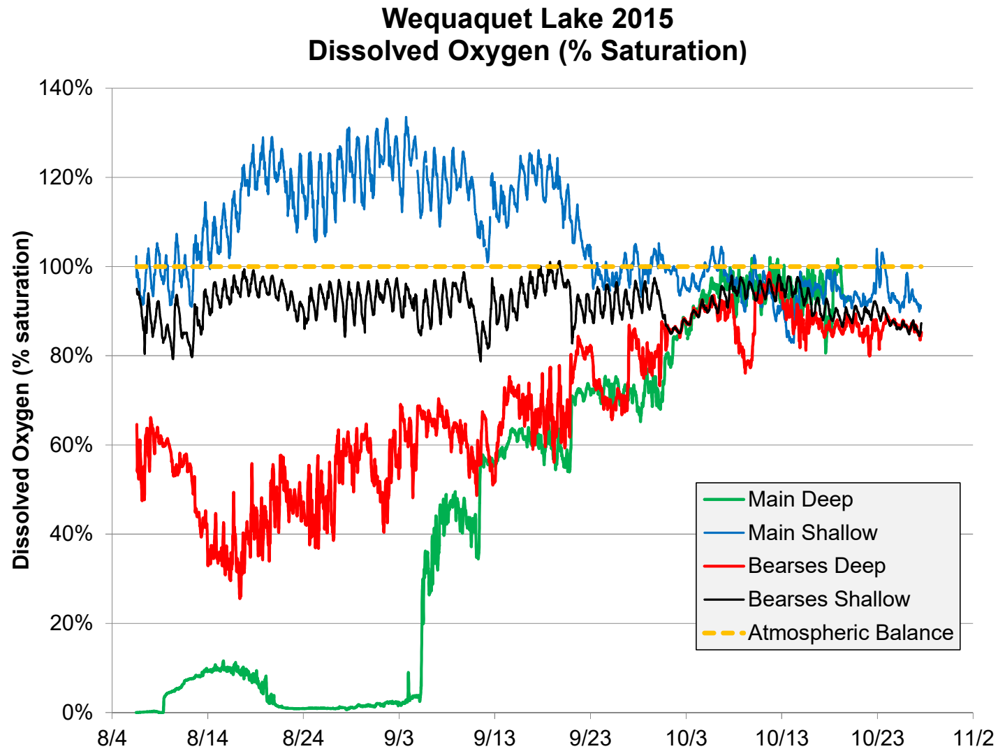
Figure 5. Lake Wequaquet 2015 DO Saturation Readings: Continuous Records in Main Basin and Bearses Pond. Recordings were collected between August 6 and October 27, 2015. Shallow readings in the Main Basin were notably above atmospheric balance from mid-August to late September. These types of conditions are generally indicative of a significant phytoplankton population. Shallow readings in Bearses Pond were generally consistent, but slightly depressed throughout the continuous recording period.
